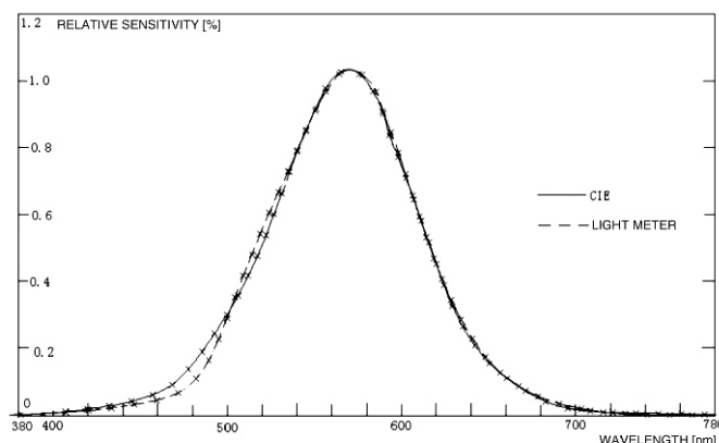
Spectral sensitivity characteristic.
